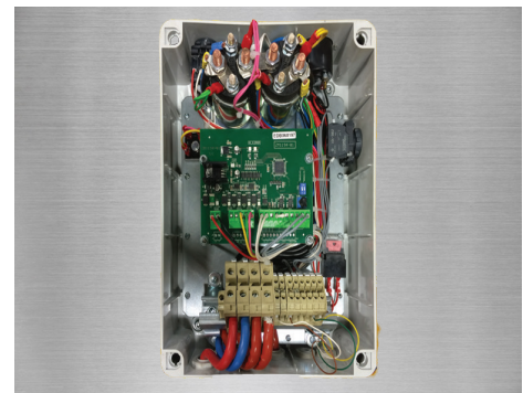
CONTROL BOX
